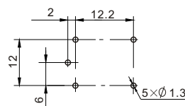
Mounting (Bottom view)
