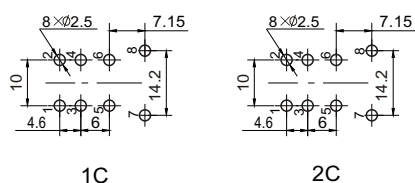
Mounting (Bottom view)
