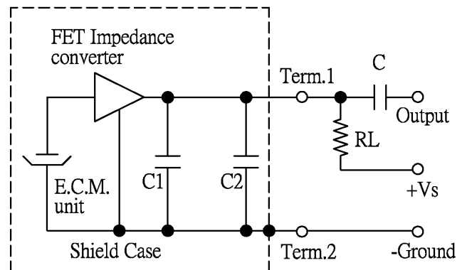
Schematic Diagram C1:33pF C2:10pF
