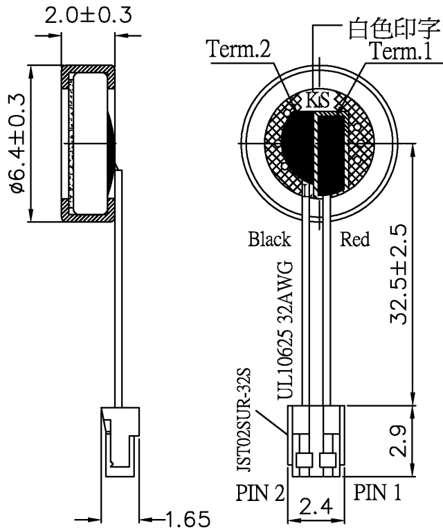
Fig D-1 Microphone with rubber holder
