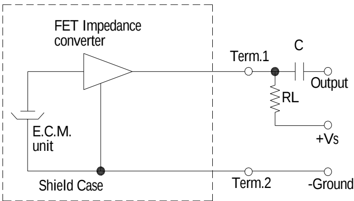
Schematic Didagram
